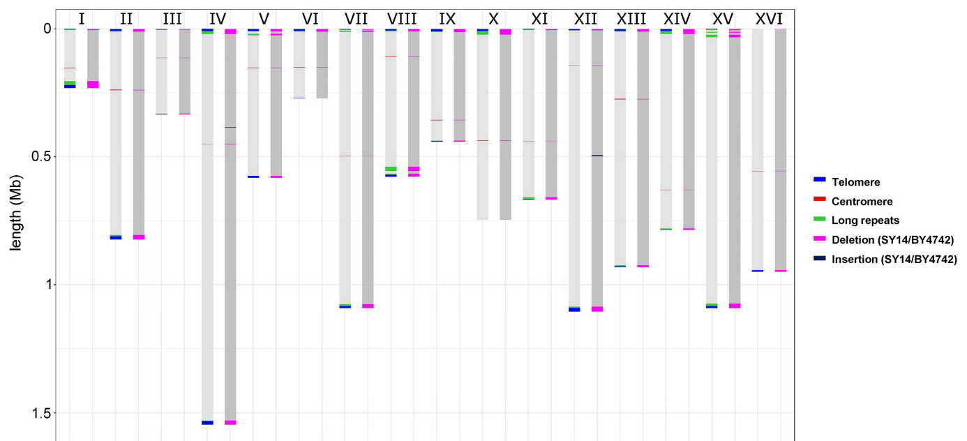
Extended Data Fig. 2 | De novo sequence comparison of BY4742 (light grey) and SY14 (dark grey) genomes. The chromosomes are labelled with Roman numerals of the yeast reference genome. The telomeres (blue), centromeres (red) and telomere-associated repeats (green) that were cut
